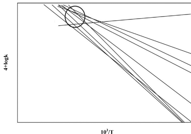
Figure 3. Arrhenius plots
