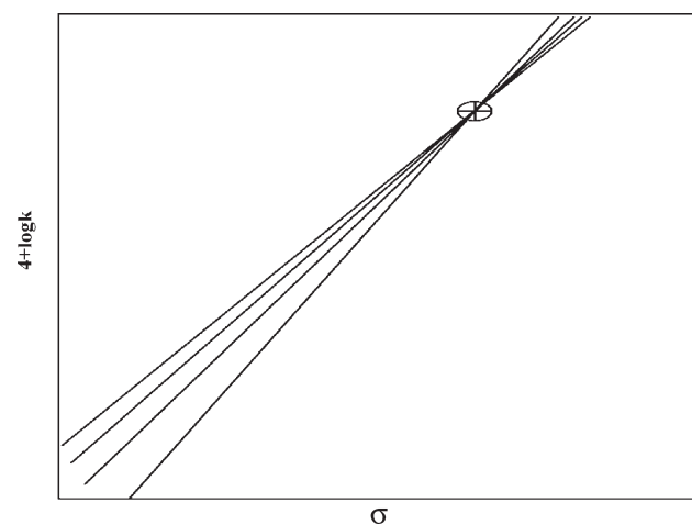
Figure 2. Hammett plots
